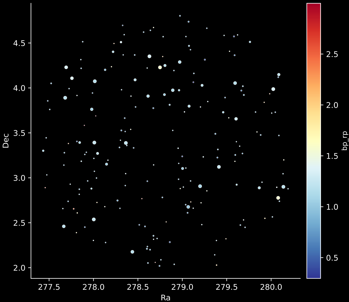
APOGEE DR17 Field: [271+63_MGA] Stars: 202
