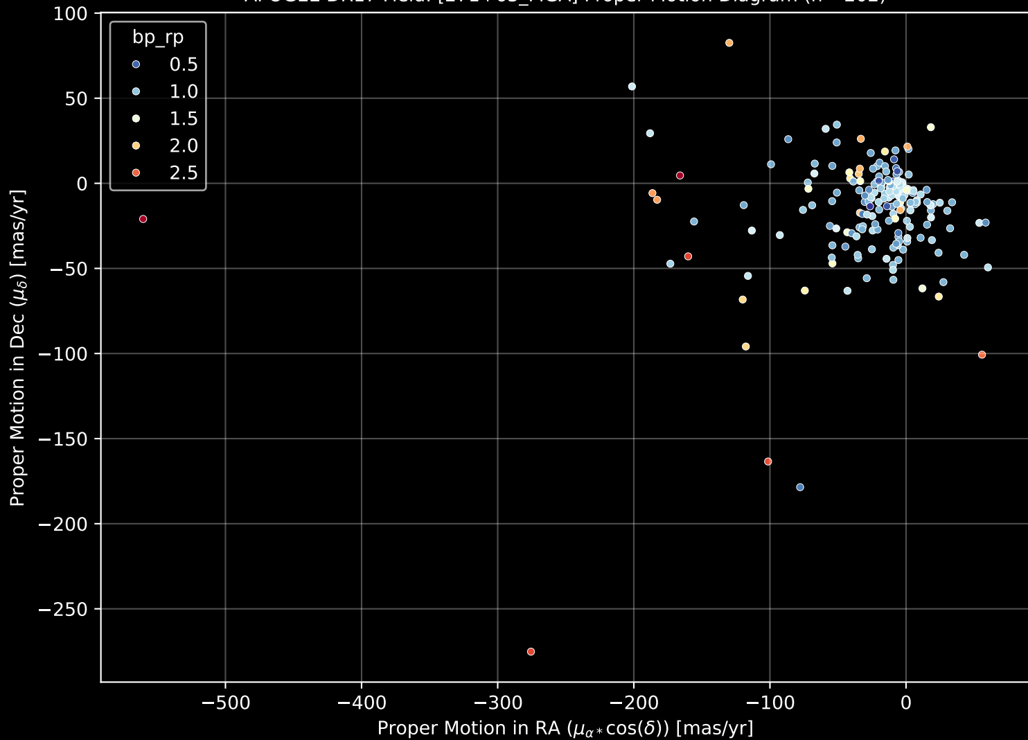
APOGEE DR17 Field: [271+63_MGA] Proper Motion Diagram (n= 202)
