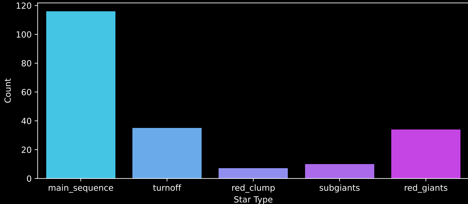
APOGEE DR17 Field: [271+63_MGA] Count plot of Star Type
