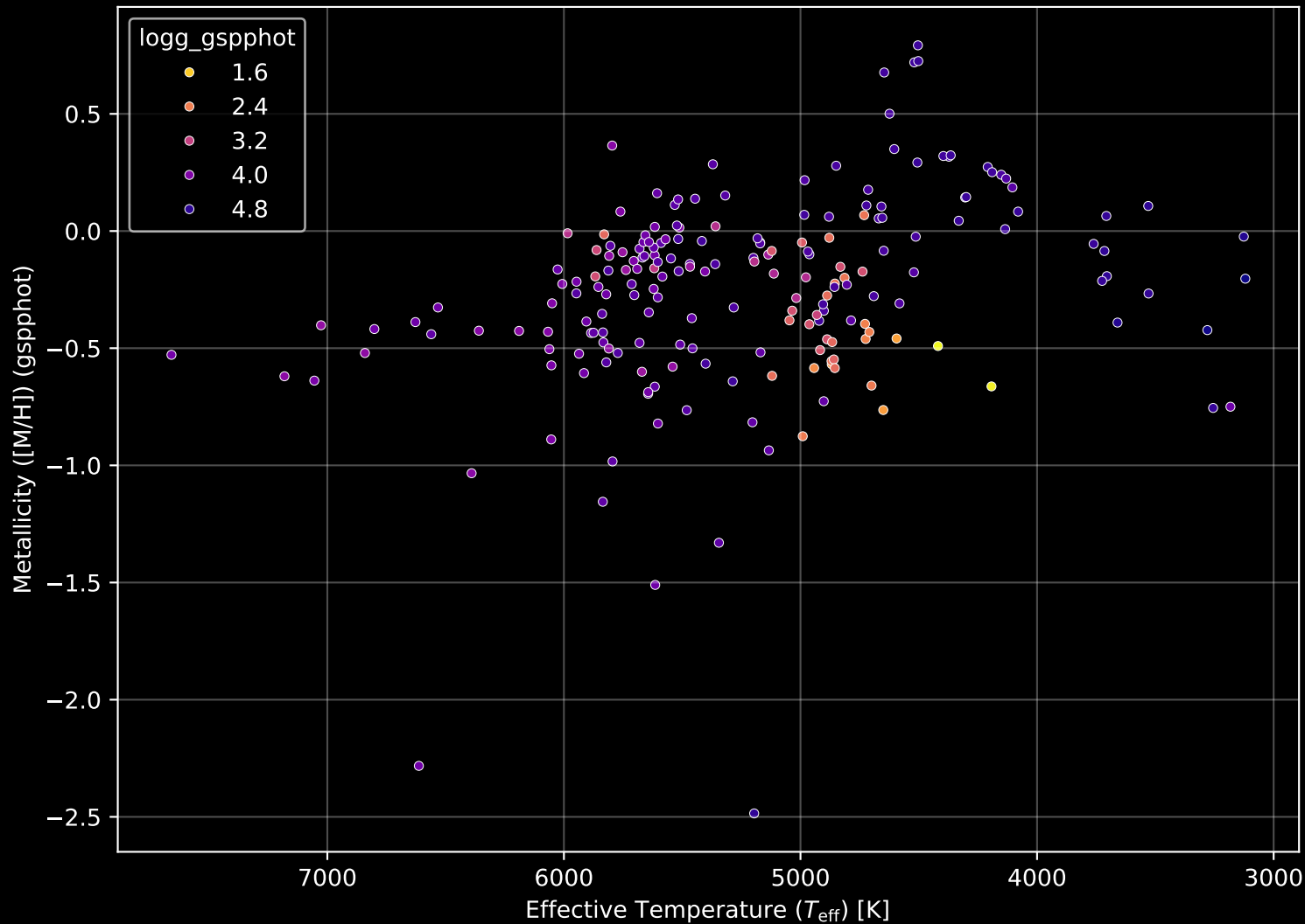
APOGEE DR17 Field: [271+63_MGA] Stellar Population Parameters (n= 202)
