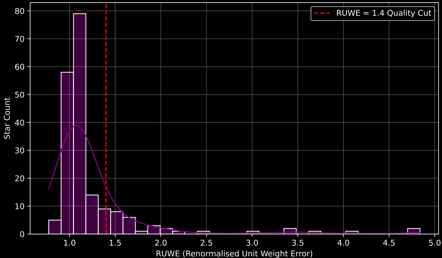
GAPOGEE DR17 Field [271+63_MGA] RUWE Distribution (n= 194)
