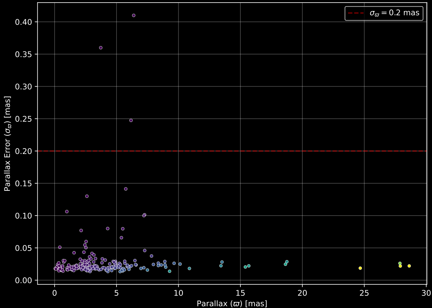
APOGEE DR17 Field: [271+63_MGA] Parallax Quality (n= 202)
