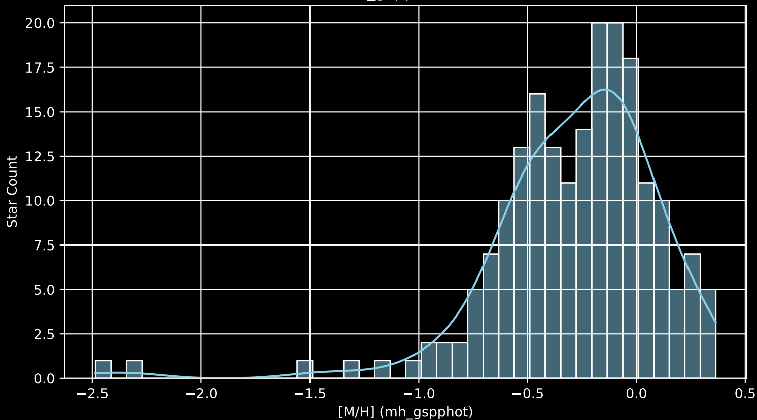
APOGEE DR17 Field: [271+63_MGA [M/H] (mh_gspphot) (n= 197)
